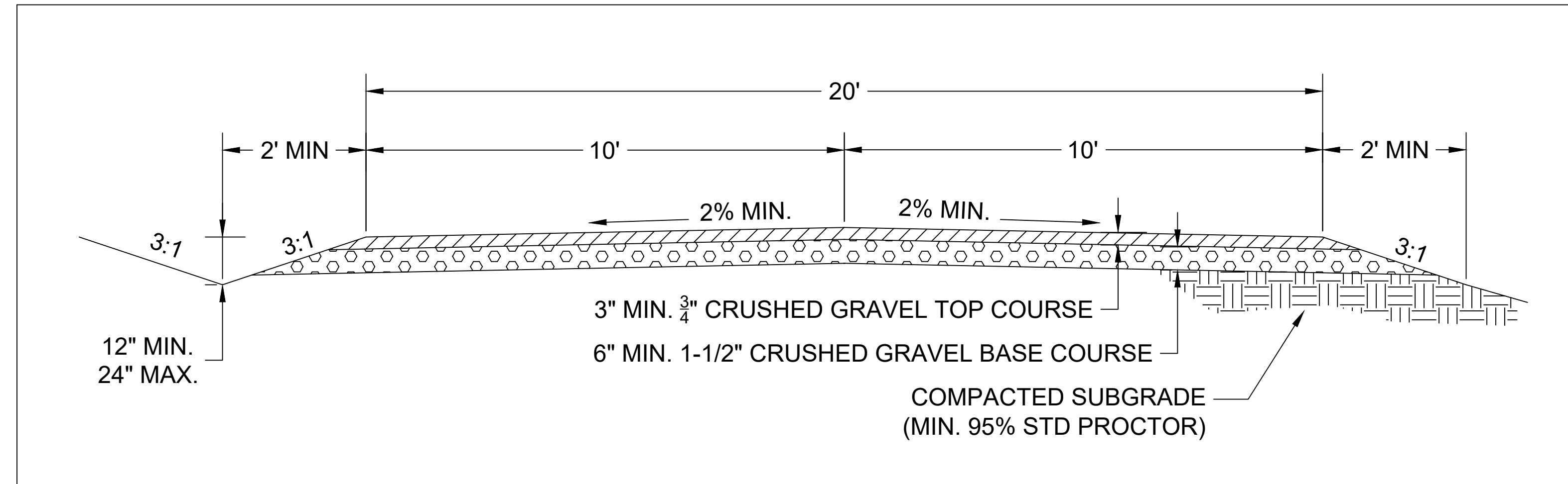
MCDEED CREEK ROAD CROSS SECTION DETAIL
