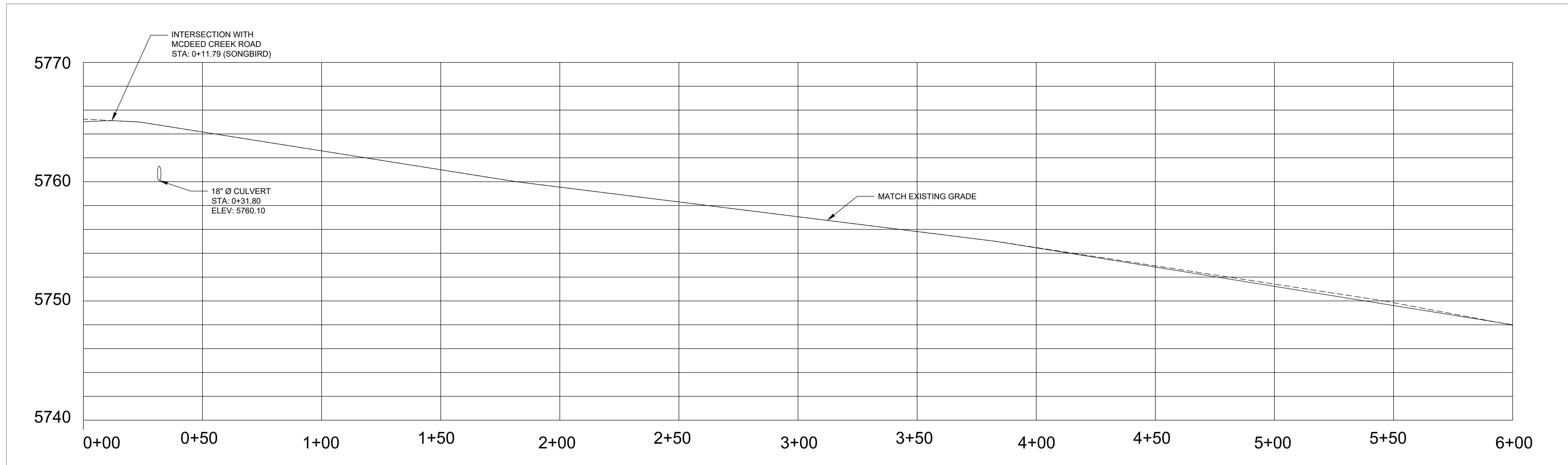
SONGBIRD WAY ROAD PROFILE
