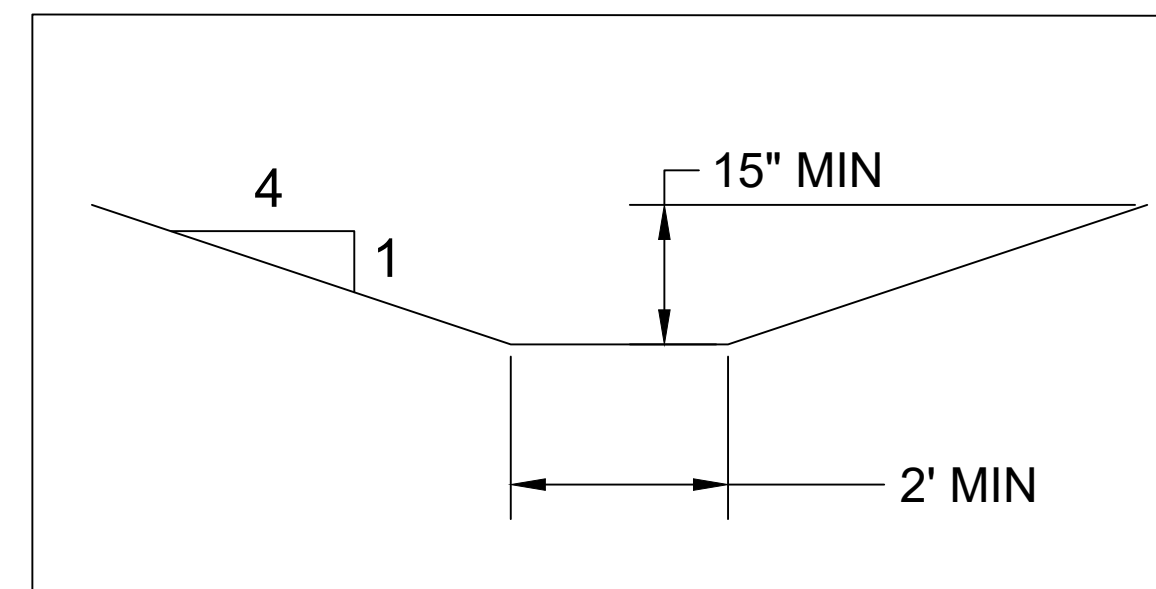
ACCESS ROAD RETENTION POND SECTION
