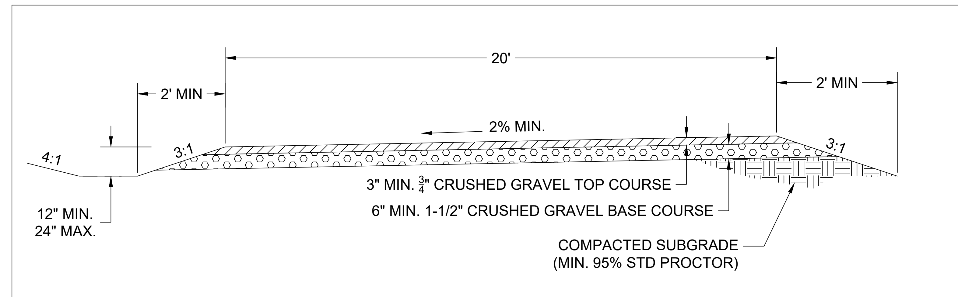
SONGBIRD WAY CROSS SECTION DETAIL
