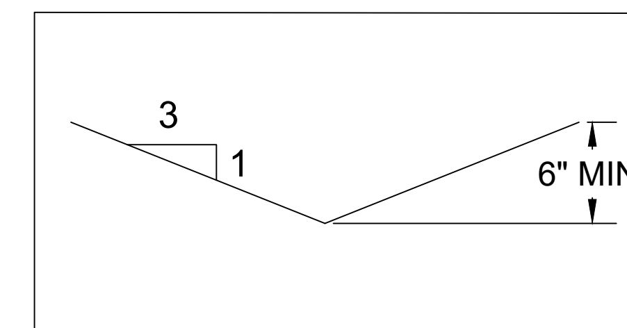
TYPICAL V-DITCH SECTION
